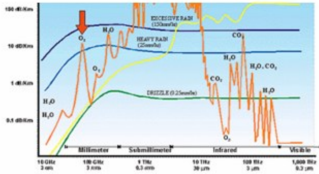
Figure 1. Atmospheric Attenuation Characteristics for Wavelengths 3 cm. to 0.3 mm
